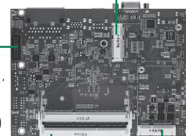
▲ Rear view Dual DDR3L SO-DIMM Full-size PCIe Mini Card (USB only) with mSATA supported
